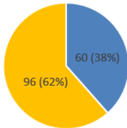
Gender distribution
