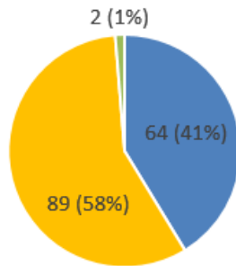
Country distribution
